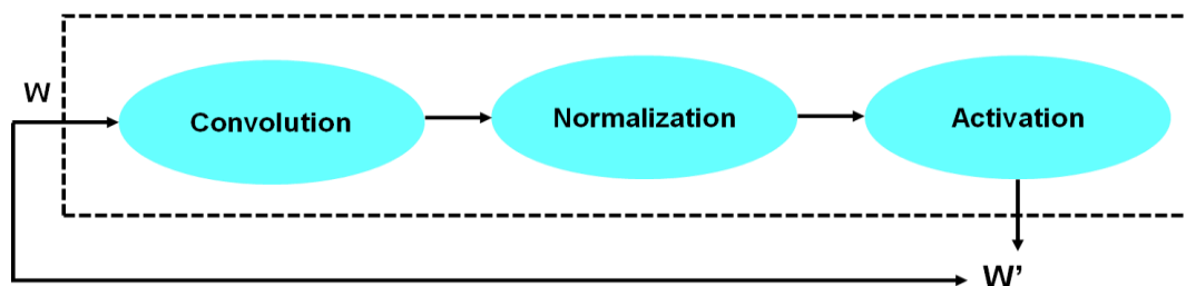
Figure 3: Residual Block.
