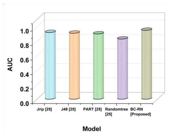
Figure 9: AUC Outcomes.
