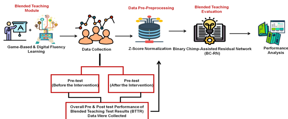
Figure 1: Method Flow.
