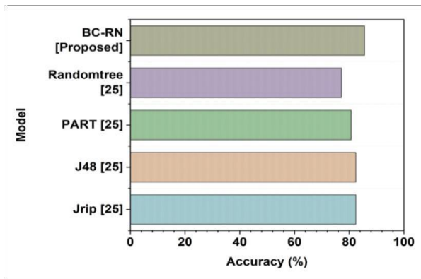
Figure 8: Accuracy Analysis
