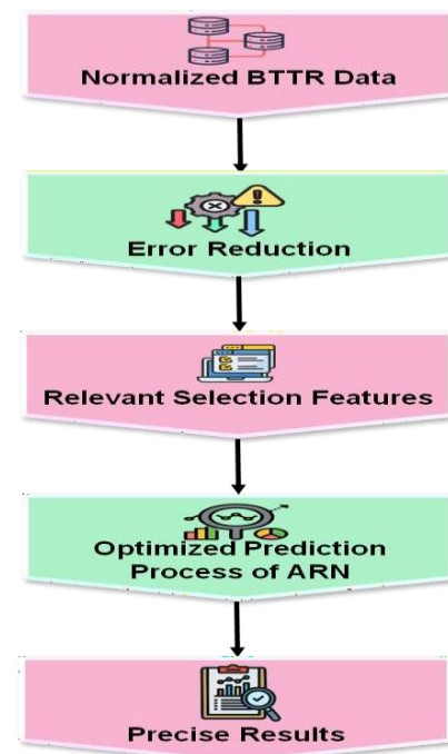
Figure 4: Optimization Process.
