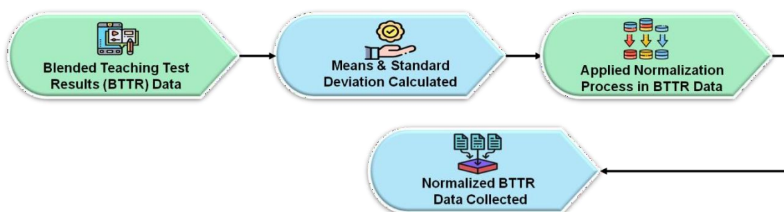
Figure 2: Normalization Process.
